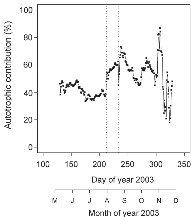
Figure 3. Autotrophic contribution to soil respiration during 2003 (Equation 1). The vertical dotted lines indicate the two summer rain events.
