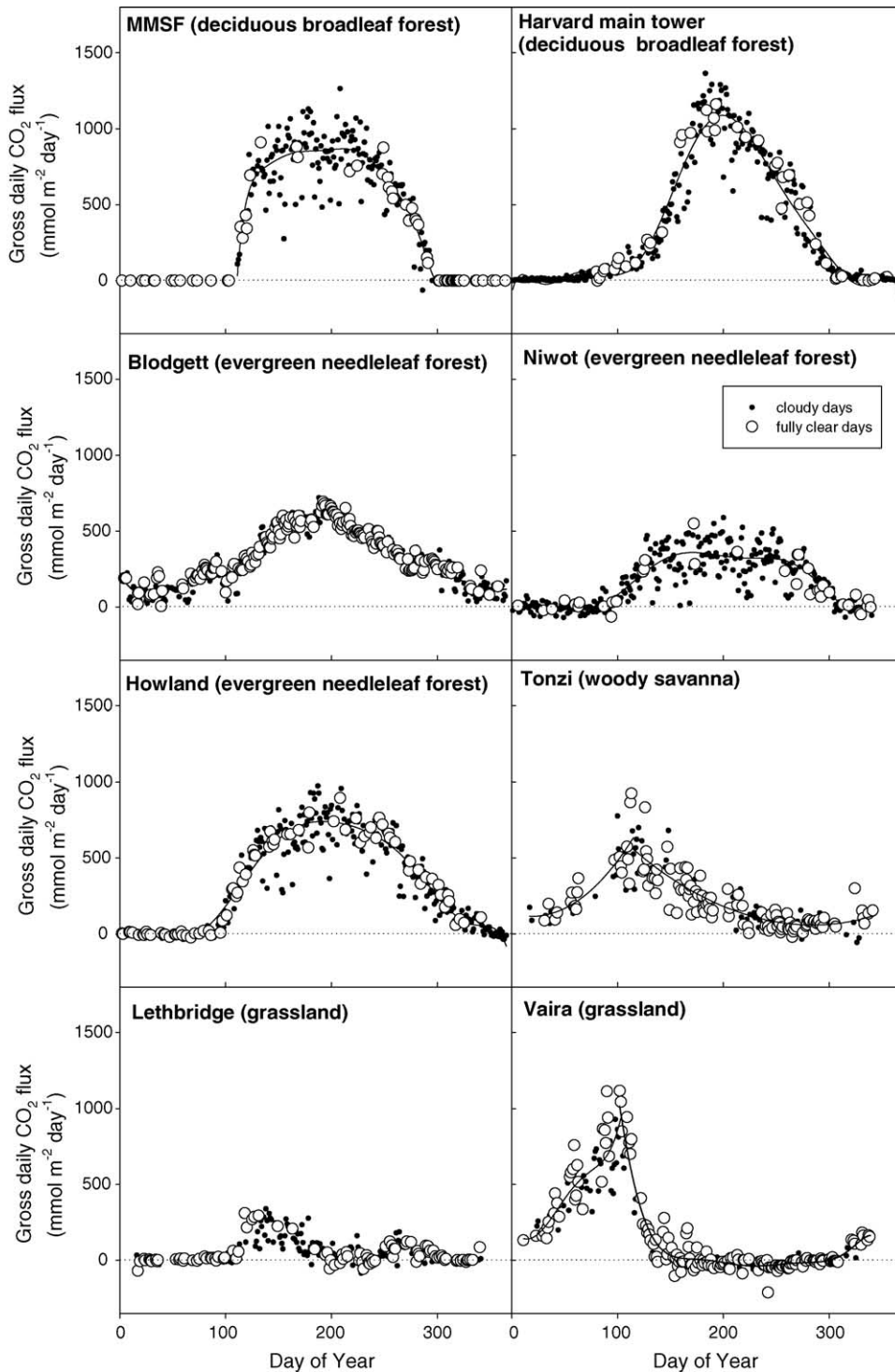
Fig. 1. Gross daily CO 2 flux (24 h totals) as a function of day of year for the eight sites in this study. Large open symbols represent clear days and small closed symbols represent cloudy and partly cloudy days.
