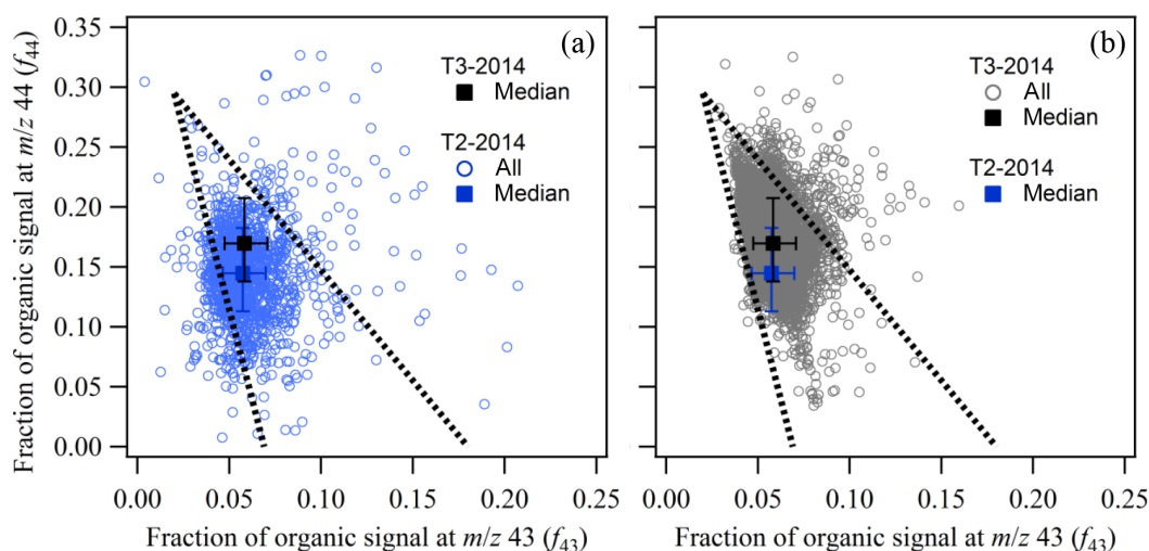
Figure 3. Scatterplot of the AMS signal fraction at m/z 44 ( f_{44} ) against that at m/z 43 ( f_{43} ). Gray and blue circles correspond to measurements at T3 and T2 during IOP1, respectively, in the wet season of 2014. For visualization purposes, the two datasets are plotted separately in panels (a) and (b). Solid squares represent median values, and whiskers represent 10 and 90 percentiles. Dashed lines delineate the region where worldwide measurements of ambient organic PM 1 commonly lie (Ng et al., 2011a).
