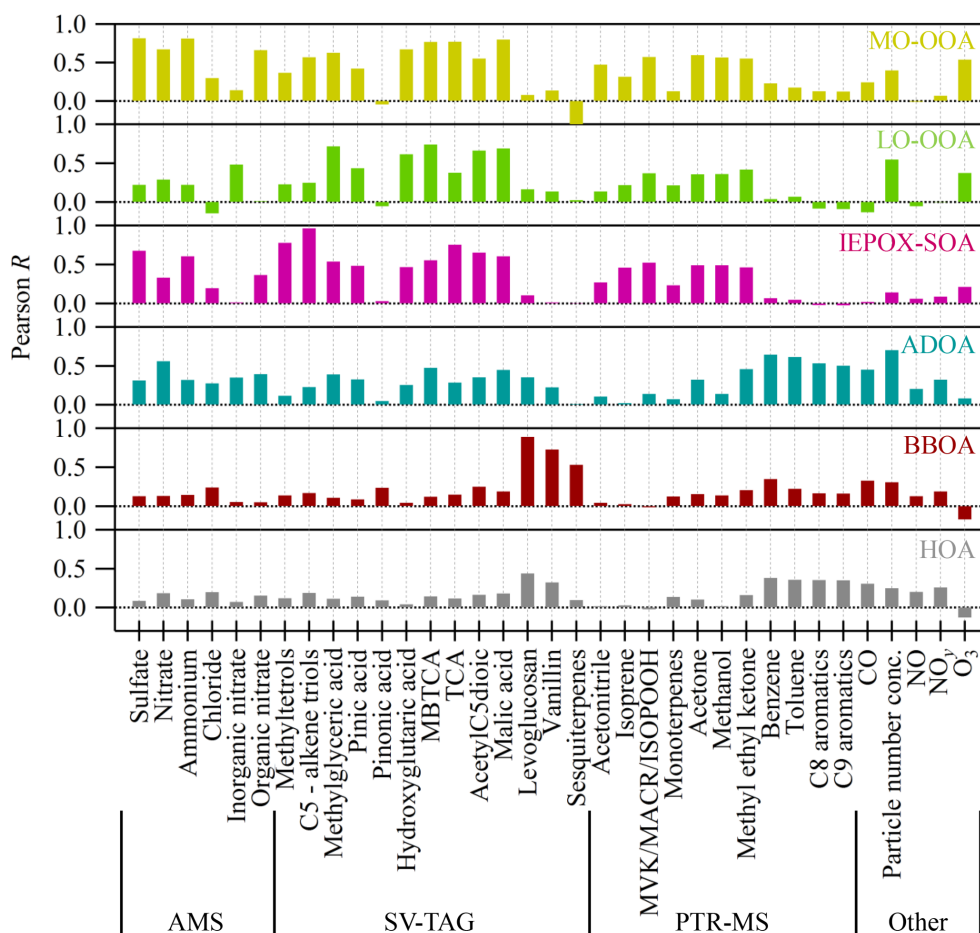
Figure 5. Column plot of Pearson R correlations between the loading of each PMF factor and values of selected measurements at T3. Abbreviations include tricarballic acid (TCA), methyl-butyl-tricarboxylic acid (MBTCA), methyl vinyl ketone (MVK), methacrolein (MACR), and isoprene hydroxyhydroperoxides (ISOPOOH). SV-TAG measurements refer to particle-phase concentrations. Isomers could not be distinguished by PTR-ToF-MS measurements; C 8 and C 9 aromatics include the xylene and trimethylbenzene isomers, respectively.
