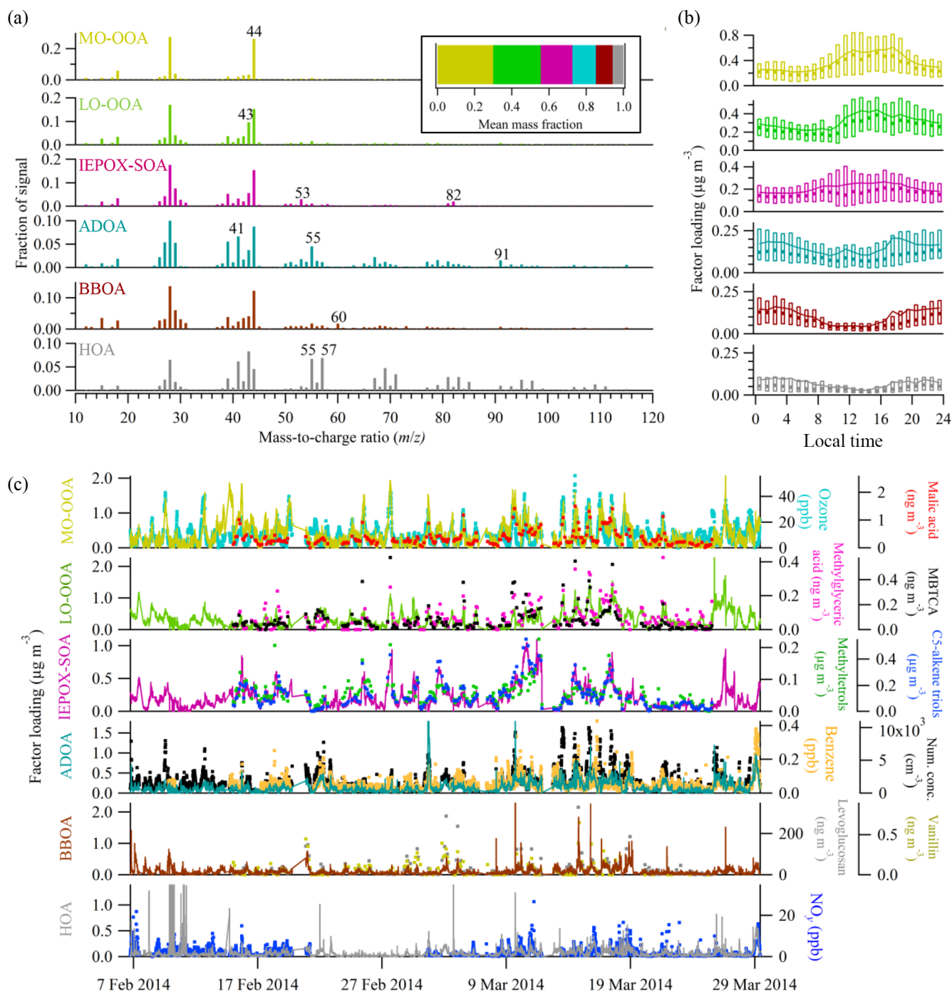
Figure 4. Results of the PMF analysis on the time series of AMS organic mass spectra collected at T3. (a) Mass spectral profile of each factor represented at unit mass resolution. The inset shows the mean fractional loading of each factor. (b) Diel trends for the loadings of each PMF factor. Local time is UTC minus 4 h. Lines represent means, solid markers show medians, and boxes span the interquartile ranges. (c) Time series of the factor loadings (left axis) and other related measurements at T3 (right axis). Methyl-butyl-tricarboxylic acid is abbreviated as MBTCA.
