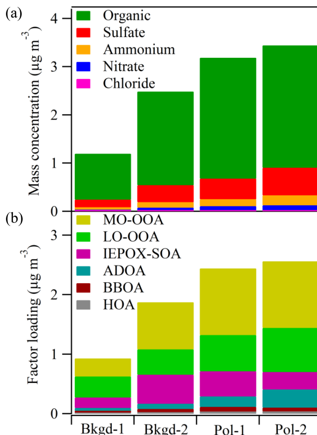
Figure 8. Characteristic PM composition of the FCM clusters as represented by coordinates of cluster centroids. (a) Mass concentrations of AMS species characteristic of each cluster. (b) PMF factor loadings characteristic of each cluster. Calculations are presented in more detail in the Supplement (Sect. S3). Values plotted are shown in Table 2.
