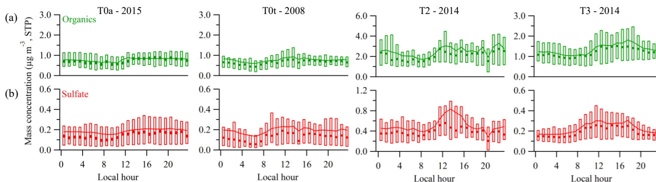
Figure 2. Diel patterns of the mass concentrations of (a, green) organic and (b, red) sulfate species during the wet season at four different sites (cf. Figs. 1 and S1). The ordinate scale for the T2-2014 panel is twice that of the other panels. Mass concentrations were corrected to standard temperature and pressure (273.15 K and 10 5 Pa) (STP). Local time is UTC minus 4 h. Lines represent means, solid markers show medians, and boxes span interquartile ranges.
