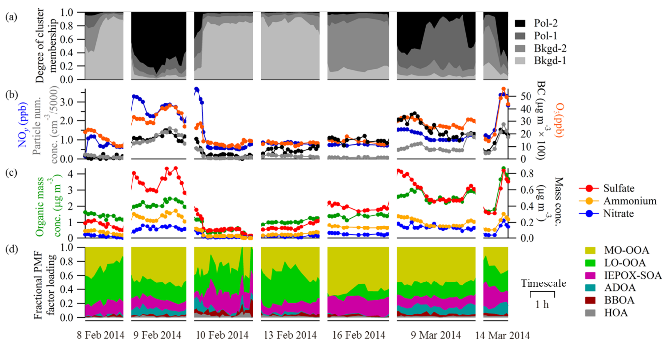
Figure 6. Results of the cluster analysis by fuzzy c-means (FCM) for afternoon periods (12:00 to 16:00 LT) are presented by several case studies. (a) The degree of membership in each of the four clusters. The sum of the degrees of membership across all clusters is unity. Background conditions are abbreviated as “Bkgd”, and polluted conditions are abbreviated as “Pol”. (b) Pollution indicators: concentrations of \text{NO}_y , \text{O}_3 , black carbon (BC), and particle number count are plotted. (c) \text{PM}_{10} mass concentrations for organic, sulfate, nitrate, and ammonium species. (d) Fractional contribution of each factor to total organic \text{PM}_{10} .
