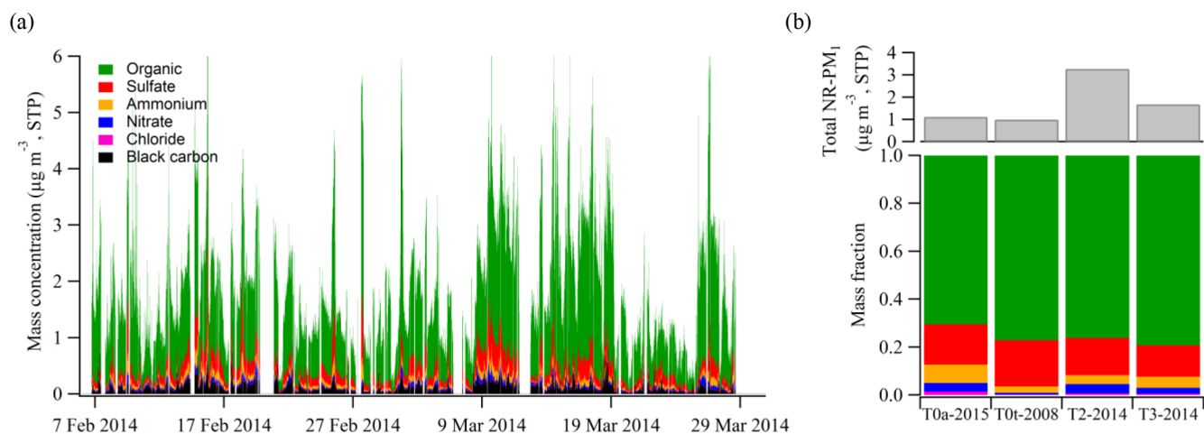
Figure 1. (a) Mass concentrations of PM 1 species at T3 during the wet season of 2014 (IOP1). Non-refractory (NR) PM 1 species of organic, sulfate, ammonium, nitrate, and chloride were measured by the AMS. Mass concentrations of black carbon were obtained by scaling aethalometer measurements by a factor of 2 based on the range of 1 to 3 for the comparison of SP2 to aethalometer measurements. The temporal trend of the two instruments agreed well. (b) Comparison of the summed mass concentrations of (top) non-refractory PM 1 species and (bottom) the mass fractions of these species at T3 and three other regional sites. T0a-2015 refers to measurements in the wet season of 2015 at the ATTO location (Andreae et al., 2015). T0t-2008 refers to the AMAZE-08 experiment, which took place in the wet season of 2008 at the TT34 location (Chen et al., 2015). T2-2014 refers to measurements made during IOP1 at a site 8 km downwind of Manaus, just across the Black River (“Rio Negro”) (Cirino et al., 2018). Measurements at T0a in 2015 and at T2 in 2014 were made by an ACSM, and measurements at T0t in 2008 and at T3 in 2014 were made by an AMS. Concentrations were adjusted to standard temperature (273.15 K) and pressure (10 5 Pa) (STP). The variability of measurements across sites is evaluated in Fig. 2.
