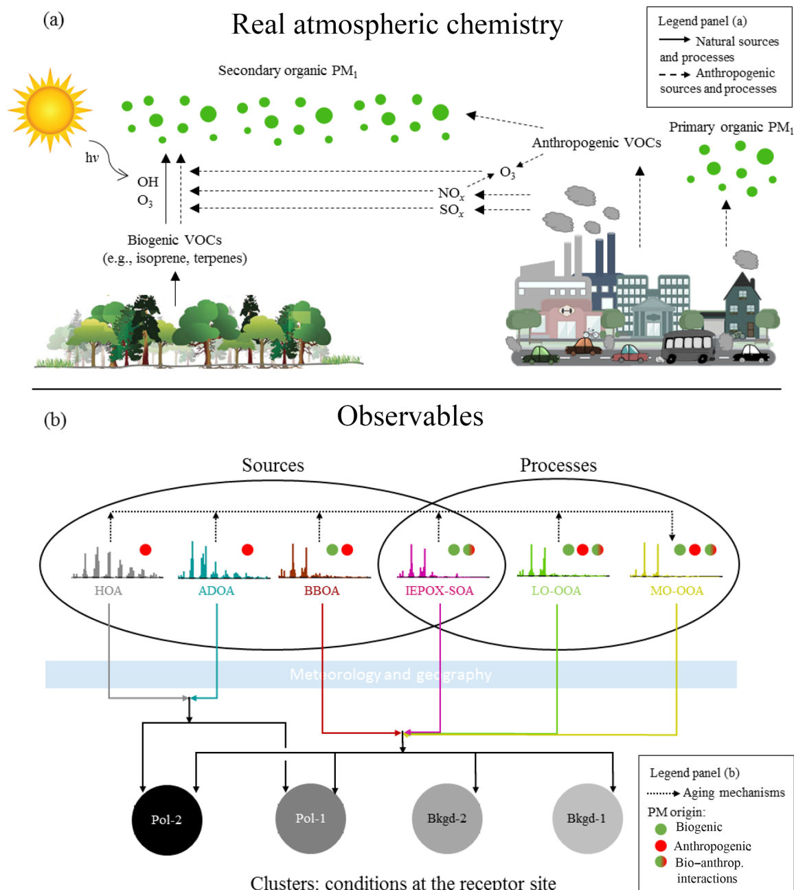
Figure 9. Schematic representation of (a) atmospheric processes, illustrated in a simplified manner, associated with the production of organic PM 1 and (b) observables of these processes as captured by the datasets and analytical approach employed in this study. In panel (a), the left side depicts the emissions of biogenic volatile organic compounds (VOCs), their atmospheric oxidation, and the production of biogenic secondary organic PM 1 . The right side depicts anthropogenic emissions of gas species and particulate matter that can alter natural atmospheric concentrations and processes. There are primary organic PM 1 emissions from traffic, cooking, and industrial activities. Anthropogenic VOCs can be precursors for the production of secondary organic PM 1 and can affect the production of ozone and hydroxyl radicals. NO x emissions directly and indirectly alter the natural pathways of PM 1 production in the atmosphere. NO x and SO x can also directly contribute to the formation of secondary inorganic PM 1 (not shown), which can in turn play a role in changing pathways of secondary organic PM 1 production. In panel (b), different PMF factors represent distinct sources and/or processes. The IEPOX-SOA factor is at the intersection of the two, as it represents both a source (i.e., isoprene emissions from the forest) and a process (i.e., photooxidation under HO 2 dominant conditions, influenced by sulfate concentrations). The dashed black line represents the natural and anthropogenic oxidative processes that transform the chemical signature of the HOA, ADOA, BBOA, IEPOX-SOA, and LO-OOA factors after sufficient atmospheric residence time into the MO-OOA factor. The clusters represent different conditions at the receptor site (i.e., T3); therefore, they incorporate the meteorological and geographical histories of the air masses that reach the site and affect the observed concentrations. The different PMF factors are associated to the different clusters (solid lines) to various extents (not detailed here for simplification purposes; cf. Fig. 8).
