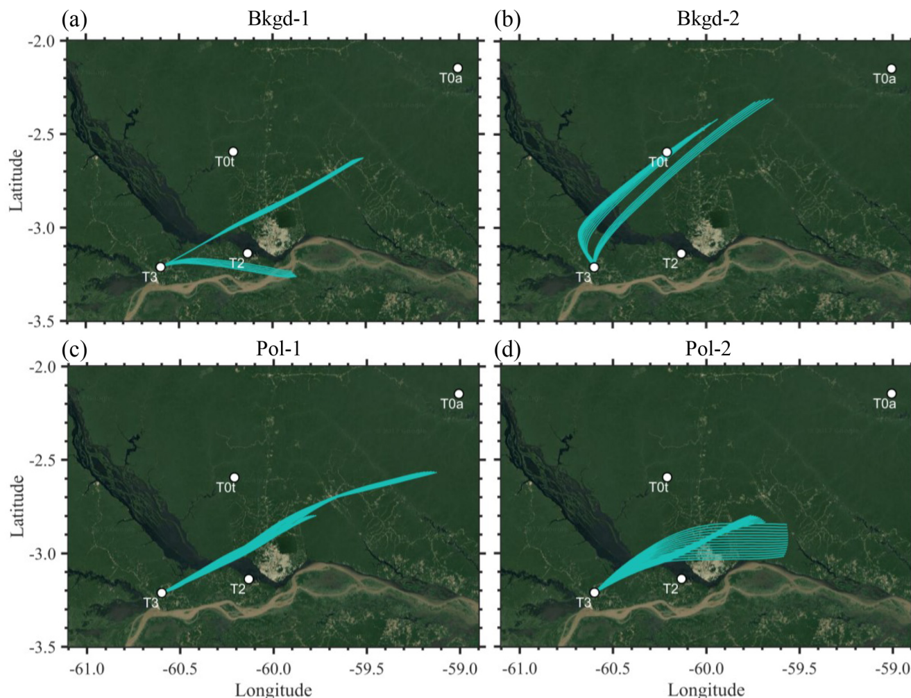
Figure 7. Air mass back trajectories associated with the four clusters of the FCM analysis for the case studies in Fig. 6. Trajectories were calculated using HYSPLIT 4 in steps of 12 min for 10 h (Draxler and Hess, 1998). Image data: Google Earth.
