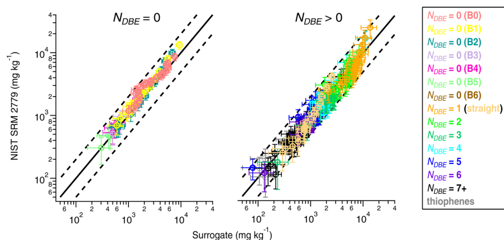
Figure 3. Comparison of mass fractions in the NIST SRM 2779 Gulf of Mexico crude oil and surrogate oil for N_{DBE} = 0 (left panel) colored by number of methyl groups ( n -alkane, B0; methyl, B1; dimethyl, B2; trimethyl, B3; tetramethyl, B4; pentamethyl, B5; and hexamethyl, B6) and N_{DBE} > 0 colored by N_{DBE} (right panel). For simplicity, all components with N_{DBE} \geq 7 are colored black. Solid lines indicate 1:1, and dashed lines indicate 2:1 and 1:2.
