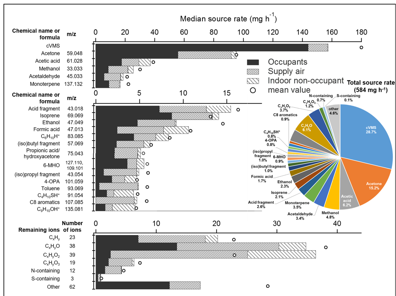
Figure 2. Median (shaded bars) and mean (circles) values of the VOC source rate ( \text{mg h}^{-1} ) measured in 18 class sessions. The mass-to-charge ratio ( m/z ) and assigned chemical formulas or names for the 20 most abundant ion/VOC groups are listed on the left of the graph. Of the remaining ions, those with known formulas are grouped by chemical composition and plotted at the bottom of the graph. The contribution of these top 20 individual ions and ion groups to the total source rate (mean value of 18 class periods) is shown in the pie chart on the right; ions with no empirical formula are summed and reported as “other”.
