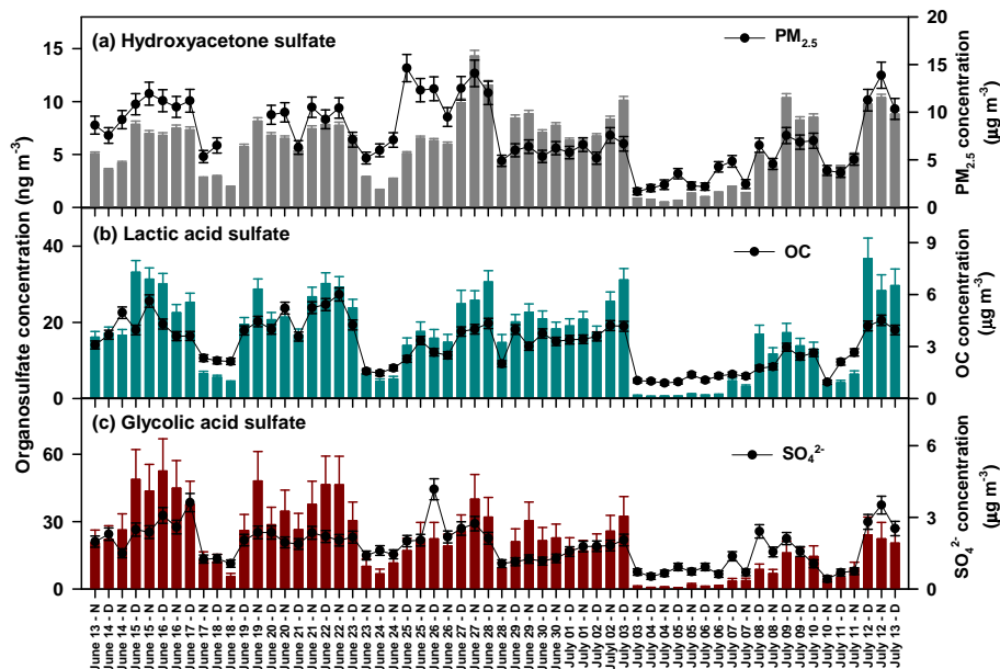
Figure 1. Concentrations of glycolic acid sulfate, lactic acid sulfate, and hydroxyacetone sulfate quantified against authentic standards, and \text{PM}_{2.5} , organic carbon (OC), and sulfate ( \text{SO}_4^{2-} ) measured at Centreville, AL, during SOAS from 13 June to 13 July 2013 on the basis of day (D; 08:00–19:00 LT) and night (N; 20:00–07:00 LT). Error bars represent the analytical uncertainty.
