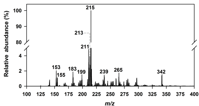
Figure 2. The mass spectrum of precursors of m/z 97 (HSO 4 - ) for the daytime sample collected on 10 July 2013 using HILIC-TQD. The 10 labelled m/z correspond to the deprotonated ions ([M-H] - ) of organosulfates with the greatest intensity.
