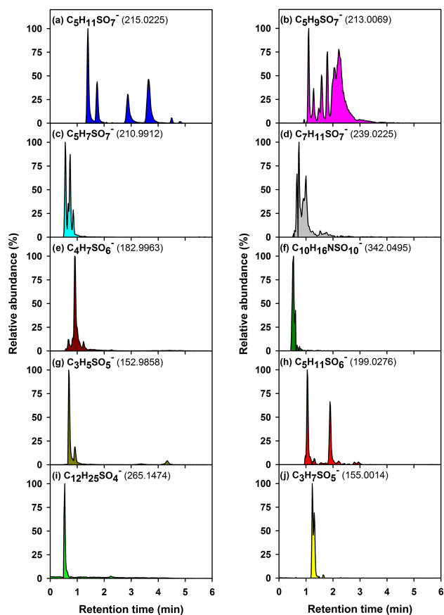
Figure 3. Extracted chromatograms for the 10 major organosulfates (monoisotopic mass \pm 0.01 Da) in the daytime sample collected on 10 July 2013 using HILIC–TOF.
