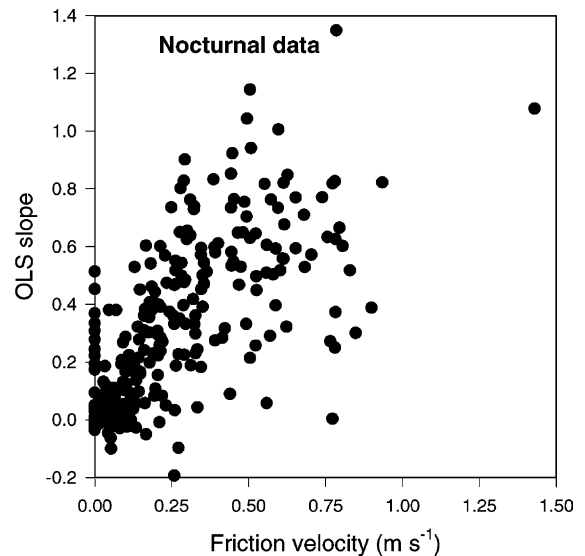
Fig. 4. The OLS slope against friction velocity ( u_* ) during nocturnal periods (net radiation less than zero). Each site-year is represented by five points, representing data sorted by friction velocity into five 20 percentile groups of half-hour data.
