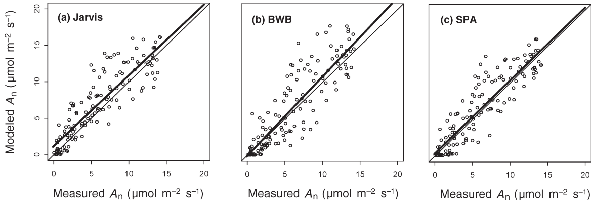
Figure 12. Measured and modeled net photosynthesis ( A_n ) with the Jarvis, BWB and SPA models for the 2000 validation period. The thin line is the 1:1 relationship. The thick line is the regression line between observations and simulations (see Table 4).
