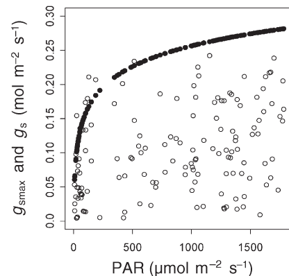
Figure 2. Relationships between photosynthetically active radiation (PAR), measured stomatal conductance ( g_s , ○) and maximum stomatal conductance ( g_{s\text{max}} , ●) modeled with the Jarvis model (Equation 11) (1999 data).
