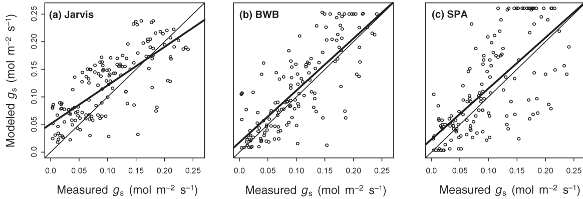
Figure 5. Measured and modeled stomatal conductance ( g_s ) with the Jarvis, BWB and SPA models for the 1999 calibration period. The thin line is the 1:1 relationship. The thick line is the regression line between observations and simulations (see Table 3).
