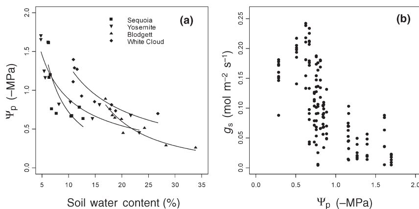
Figure 1. Relationships between (a) soil water content at 50-cm depth and predawn leaf water potential ( \Psi_p ) and between (b) \Psi_p and stomatal conductance ( g_s ) at four sites during 1999 and 2000. Lines were calculated with Equation 10, see Table 1.
