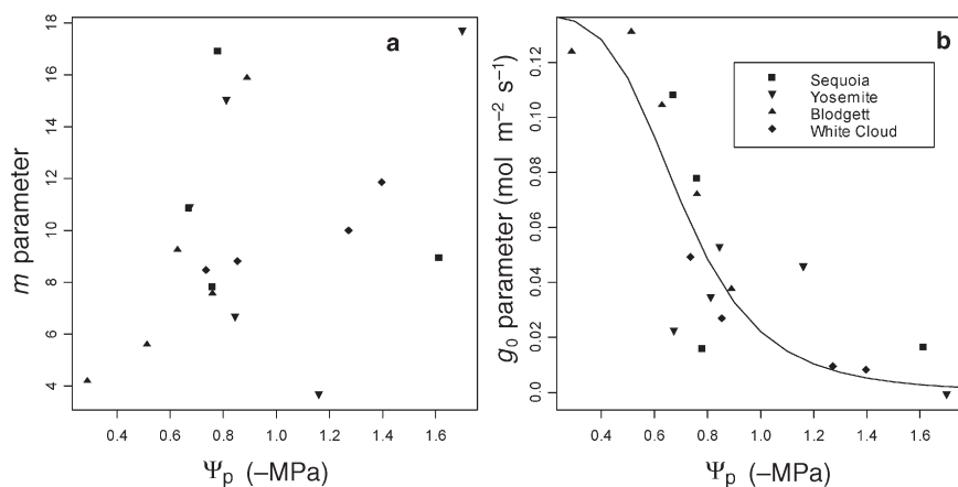
Figure 3. Relationships between parameters m (Figure 3a) and g_0 (Figure 3b) of the BWB model and predawn leaf water potential ( \Psi_p ) at the four sites during the 1999 period. The line in Figure 3b was calculated with Equation 12 ( r^2 = 0.71 ).
